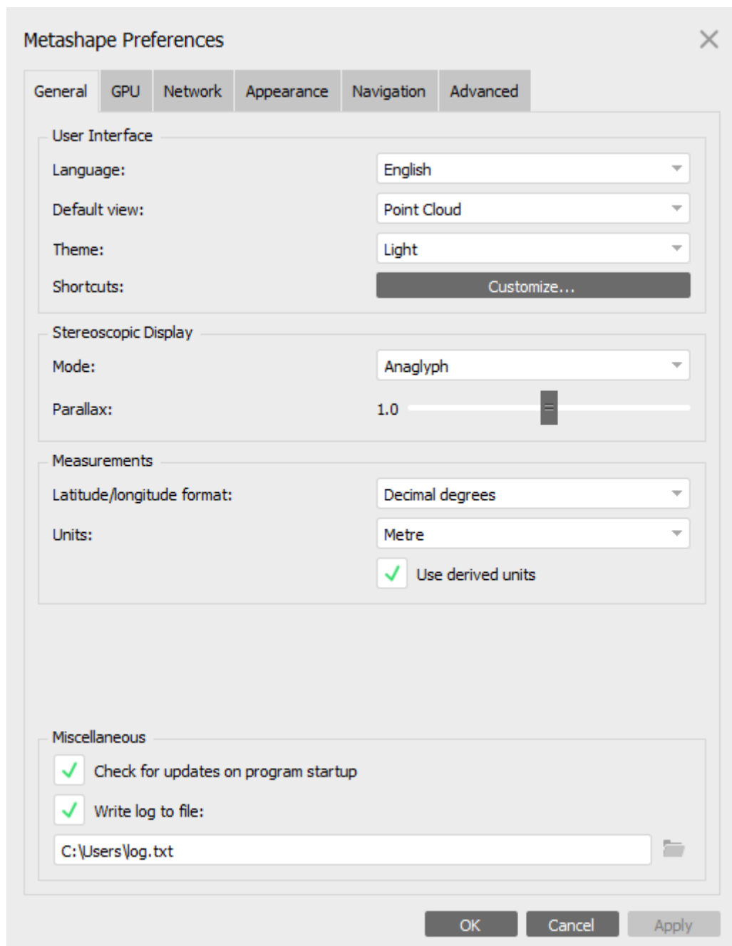
General tab
