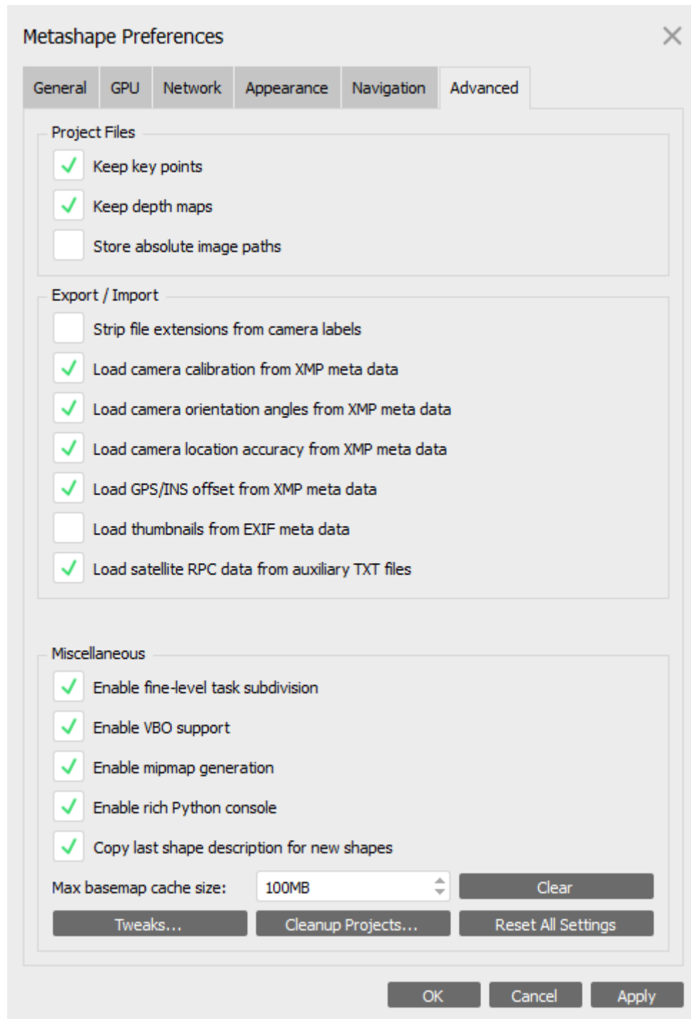
Advanced tab
